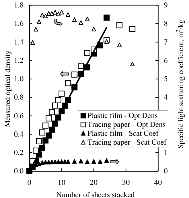
Fig.2 Comparison in optical density measured by Elrepho-type reflectometer between plastic film and tracing paper stacks.
