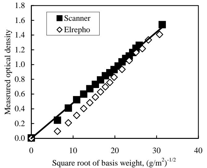
Fig.4 Comparison in optical density of tracing paper stack.
