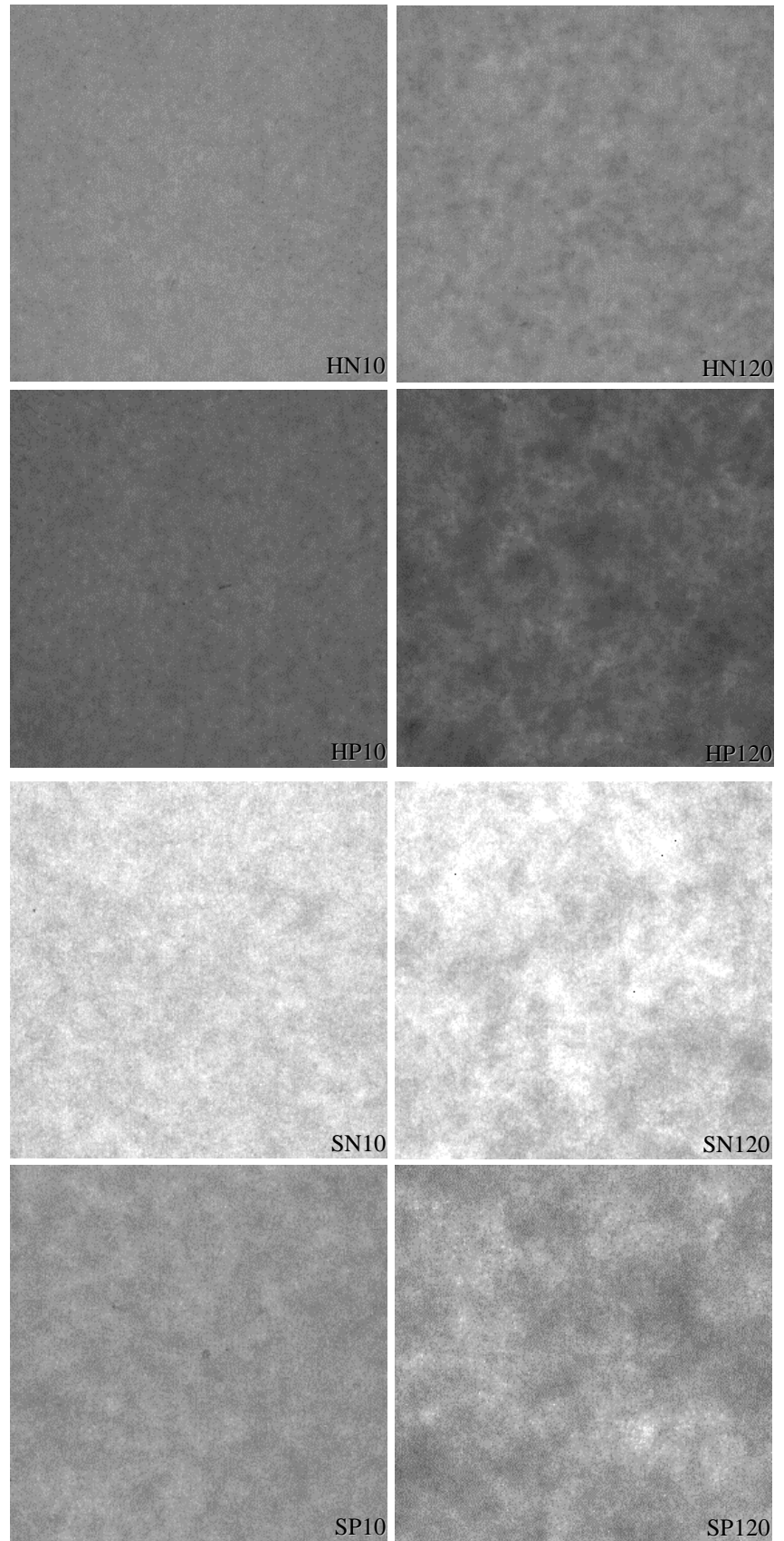
Fig.5 Light transmission images of handsheets made from bleached hardwood kraft pulp. Details are in Table 3.
