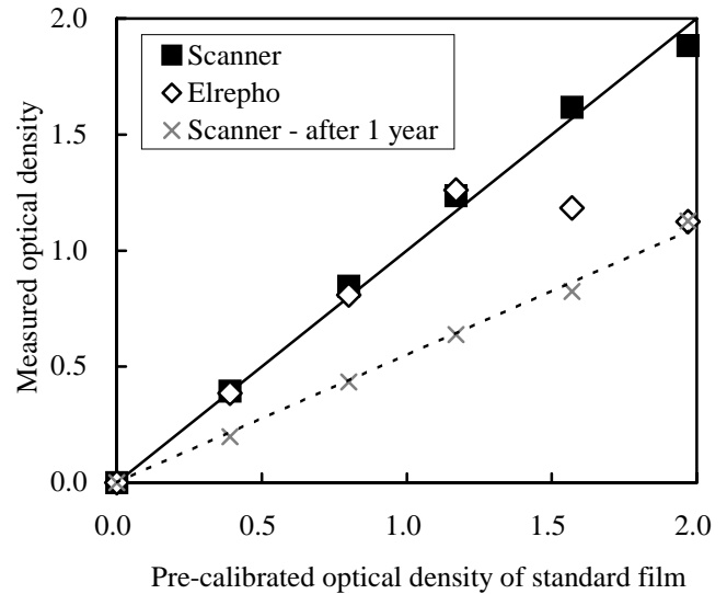
Fig.1 Comparison in optical density of the standard film measured between by scanner and by Elrepho-type reflectometer
