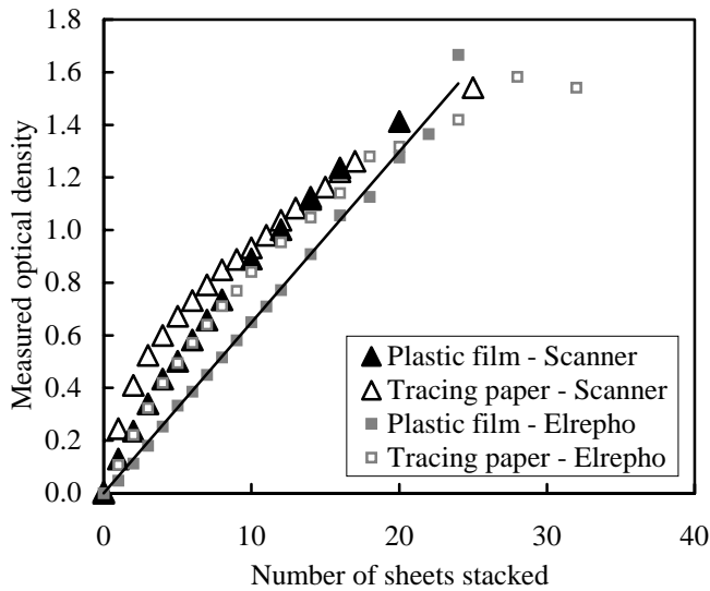
Fig.3 Distortion of scanner output. For the same material stacks, scanner optical density curves upward.
