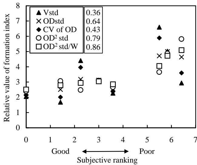
Fig.6 Formation indices and their Kendall's coefficient of correlation. OD^2 -based indices shows better correlation.
